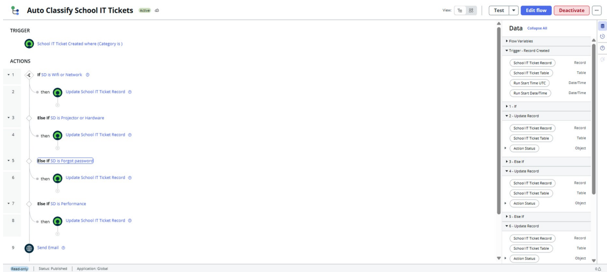
Figure 1: Flow Designer implementation of the automatic classification requirement.
